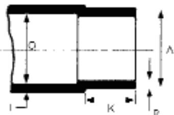
MALE (FITTING)
